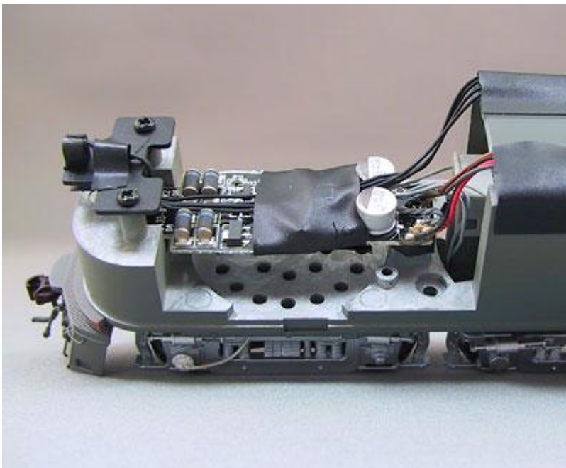
Forward speaker cut-out
