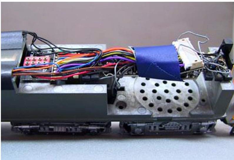
Aft speaker cut-out
