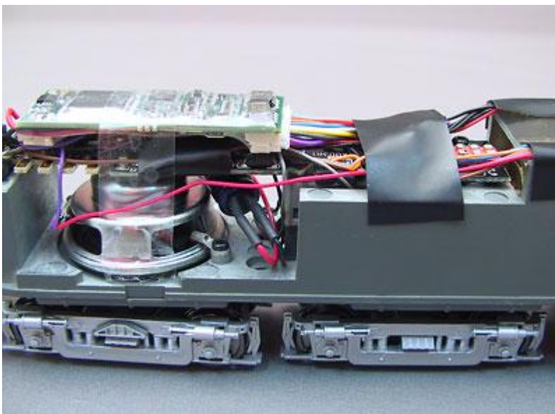
1.22" HB speaker, aft location with Revolution-U connected to the loco "Quick Plug"
