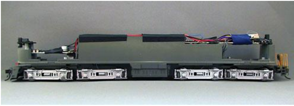
Loco before installation
