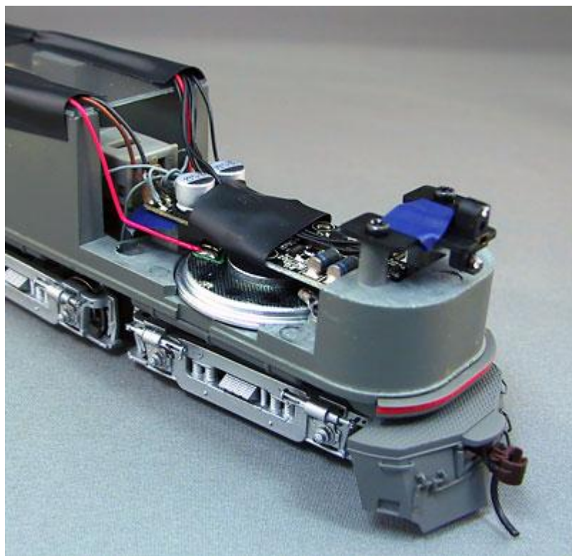
Forward 1.25" speaker installed
